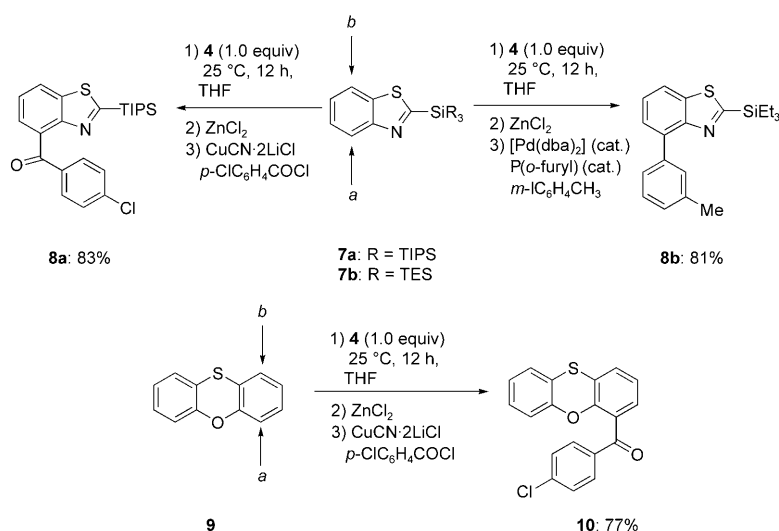
Scheme 2. Regioselective almination of the benzothiazoles 7a and 7b and phenoxathiine ( 9 ) with the aluminum base 4 and subsequent transmetalation with \text{ZnCl}_2 , followed by copper-mediated acylation or palladium-catalyzed cross-coupling. dba = dibenzylideneacetone, TES = triethylsilyl, TIPS = triisopropylsilyl.
