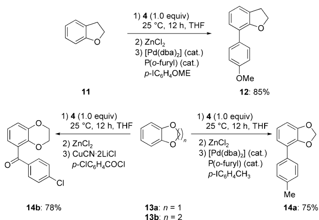
Scheme 3. Alumination of substrates with annelated oxygen-containing rings and subsequent transmetalation with \text{ZnCl}_2 , followed by copper-mediated acylation or palladium-catalyzed cross-coupling.
