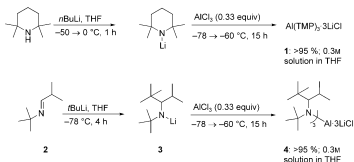
Scheme 1. Preparation of the aluminum trisamide bases 1 and 4 .
